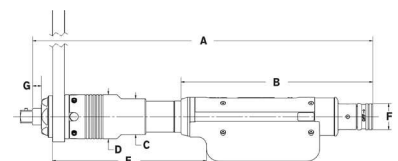
Standard Spindle (A) Models
