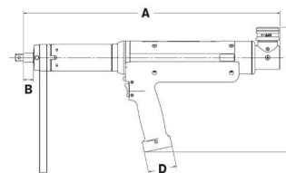
Extended Ergo Drive Top Exit (AVT) Model
